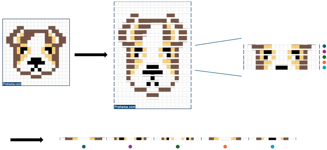
Figure 9: Visualization of how images are converted into vectors
