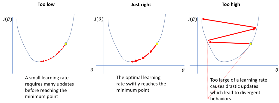
Figure 15: A demonstration of how different learning rates affect convergence of a loss function (in this graphic represented as J(\theta) ).
