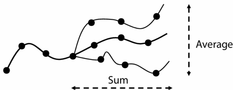
Figure 29: A visualization of what the Q-function takes into account. It averages the rewards from time t and forward across considers many paths that policy \pi_\theta could theoretically take. The output of a Q-function is called a Q-value. It signifies the “quality” of the given state-action pair.
