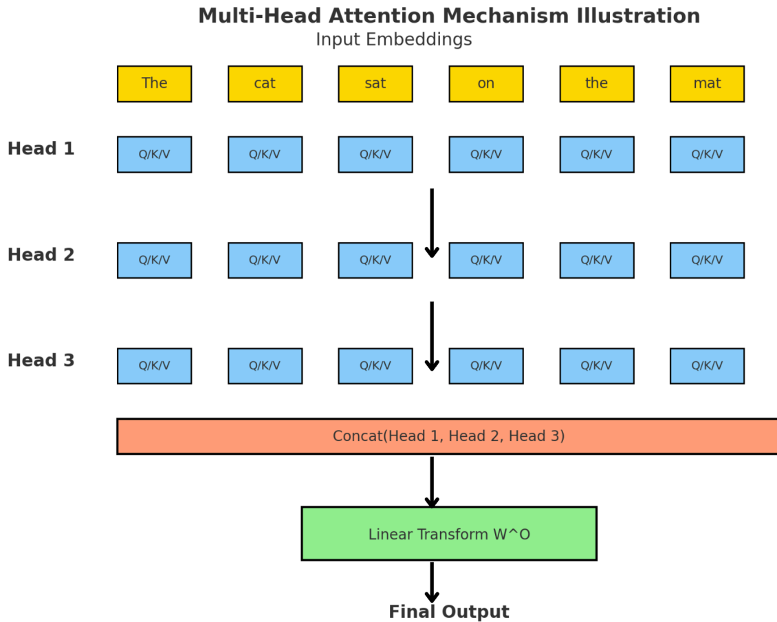
Figure 30: Multi-Head Attention Mechanism: Each head captures unique relationships and combines them for comprehensive context.
