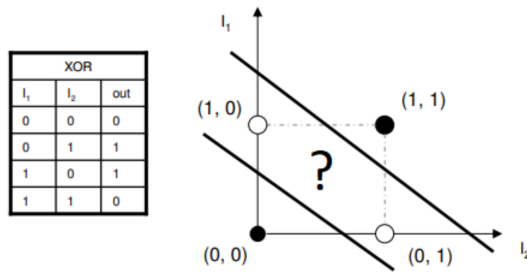
Figure 11: Illustration of the XOR function, and how you cannot draw a single line that separates the classes (white and black dots).
