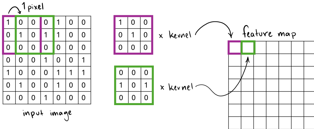
Figure 19: Illustration depicting a stride of 1 pixel
