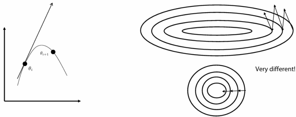
Figure 28: There are a few items in this diagram. The parabola and tangent show the issues of large gradient steps when you have only a monte-carlo approximation to the true gradient. You can wildly overshoot where you should be ( \theta_{i+1} ). The dimensions of the stretched oval represent the parameters of the policy, and how steps in the wrong direction can be disastrous since the policy is very sensitive to small parameter shifts. What we don't have in RL is an easy objective to optimize on like the circle. These problems together are why NPG is useful.
