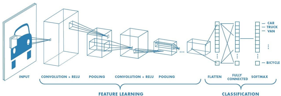
Figure 22: Illustration of complete architecture of CNN
