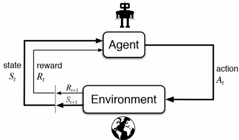
Figure 27: An illustration showing how the agent and environment communicate through actions, states, and rewards in a traditional RL setting. The subscript t is for timestep.
