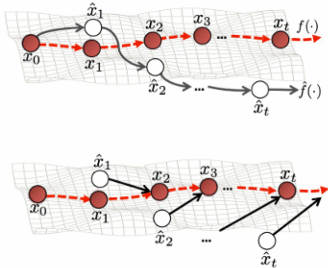
Figure 26: A visualization of how DAgger helps keep the agent performing well. We first see the agent ( \hat{x} ) deviate from the expert ( x ), but we then take these observations of where the agent failed and give it instructions on how to get back on track. With enough iterations, a lot of failure cases can be mitigated.
