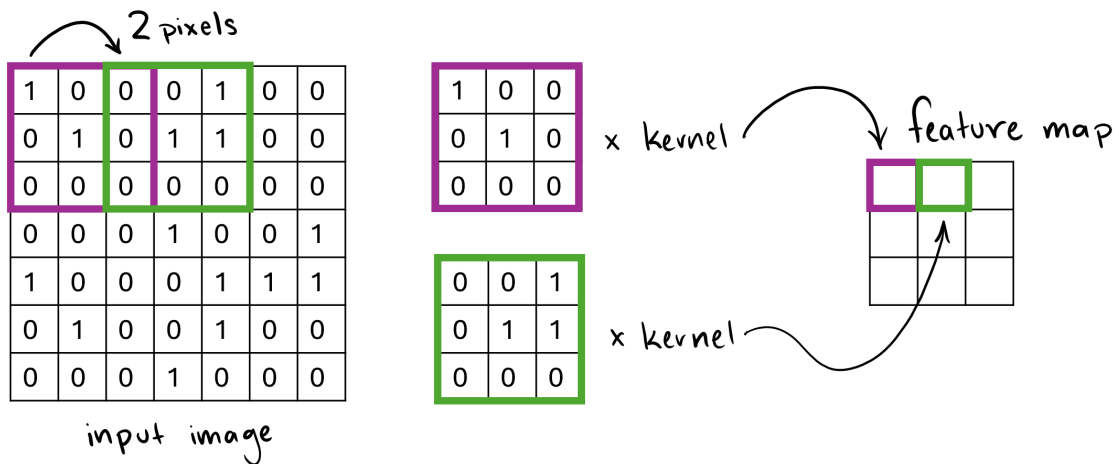
Figure 20: Illustration depicting a stride of 2 pixels
