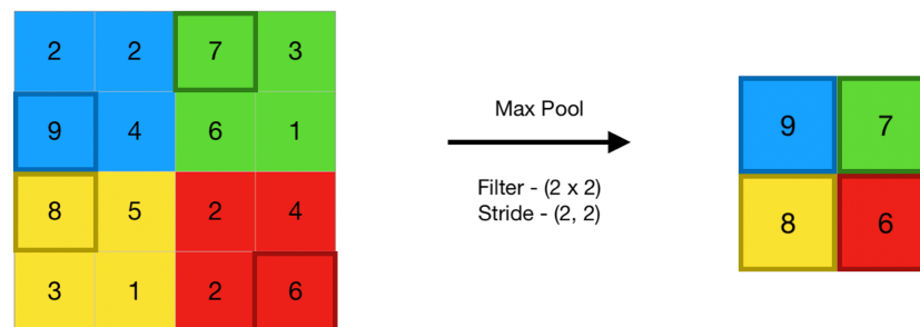
Figure 21: Illustration of the max pooling operation
