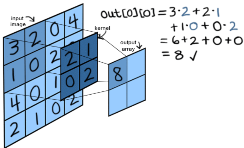
Figure 18: Illustration of the work done in a convolutional layer
