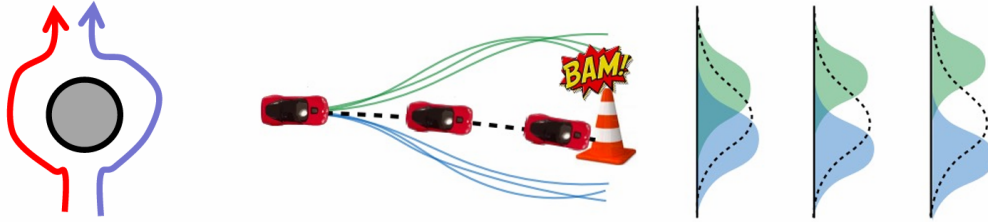
Figure 24: An illustration demonstrating the issues that arise from mode-averaging within behavior cloning algorithms. The green and blue peaks represent choosing to go left or right around the obstacle, and the black dashed line represents what a simple policy will converge on.
