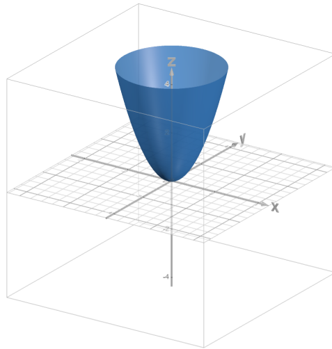
Figure 13: Illustration of the function f(x, y) = x^2 + y^2
