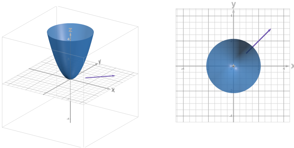
Figure 14: Illustration of the function f(x, y) = x^2 + y^2 , with a vector showing the direction of steepest ascent from point (1, 1)
