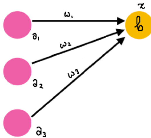
Figure 10: An illustration of weights and biases connecting the first layer of our neural network to the first neuron of the second (hidden) layer.
