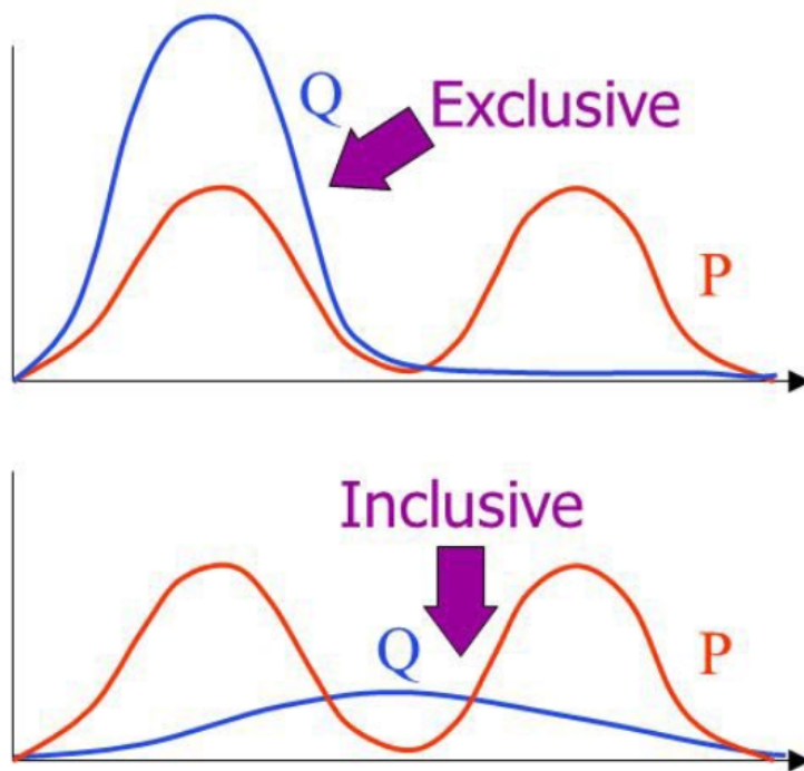
Figure 25: The blue curve is our single-mode Gaussian decision policy and the bimodal orange line is our expert policy (can go left or right around the tree). The top graph shows what we would like to happen, which is choosing a mode and sticking with it. However, the bottom graph shows what actually happens when we minimize forward KL divergence. This is mode-averaging behavior (crashing into the tree).
