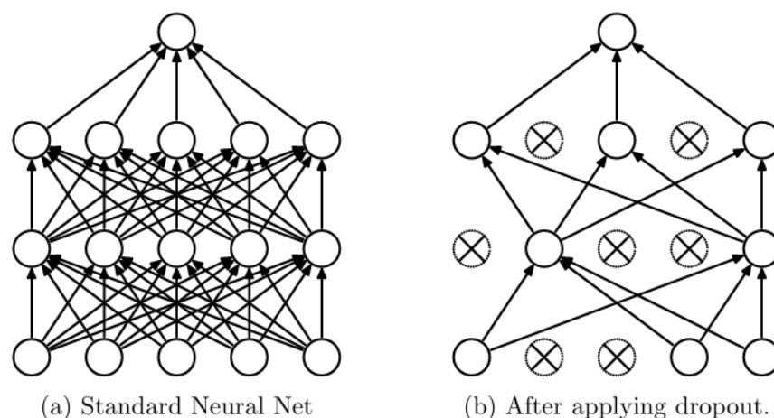
Figure 16: Visualizing dropout in a fully connected neural network
